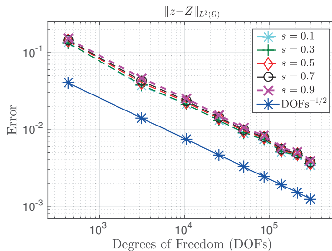
FIGURE 3. Computational rates of convergence for the fully discrete scheme proposed in Section 6 on anisotropic meshes for n = 2 and s = 0.1 , s = 0.3 , s = 0.5 , s = 0.7 and s = 0.9 . The figure shows the decrease of the L^2 -norm of the error for the optimal control with respect to \#\mathcal{T}_\gamma . In all the cases we recover the rate (\#\mathcal{T}_\gamma)^{-1/2} .
