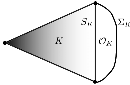
FIGURE 1. An element K , for n = 2 , such that K \cap \partial\Omega_{\mathcal{T}} \neq \emptyset and the corresponding curved region \mathcal{O}_K : S_K denotes the side of K that lies on \partial\Omega_{\mathcal{T}} , \Sigma_K the corresponding arc formed by the curved boundary \partial\Omega and \mathcal{O}_K the region bounded by \Sigma_K and S_K .
