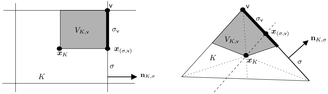
FIGURE 3. Notations for MPFA-O schemes defined on Cartesian ( left ) and simplicial ( right ) meshes.
