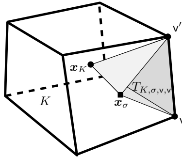
FIGURE 5. Definition of tetrahedron T_{K,\sigma,v,v'} in a mesh cell K .
