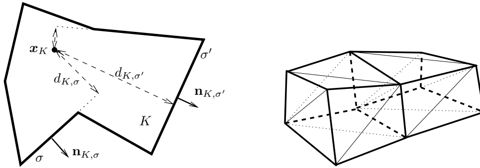
FIGURE 1. A cell K of a polytopal mesh (left). Two neighbouring generalised hexahedra (right).
