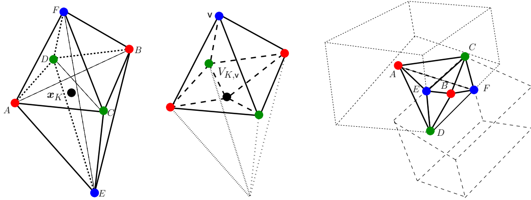
FIGURE 4. Left : octahedral cell K for the CeVeFE-DDFV scheme. Center : illustration of V_{K,v} . Right : construction of a degenerate octahedron from a non-conforming hexahedral mesh in a heterogeneous medium ( CDEF is the intersection of the boundaries of two non-matching hexahedral cells).
