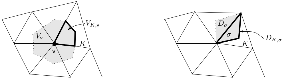
FIGURE 2. Partitions for mass-lumping of the \mathbb{P}_1 (left) and non-conforming \mathbb{P}_1 (right) finite element methods.
