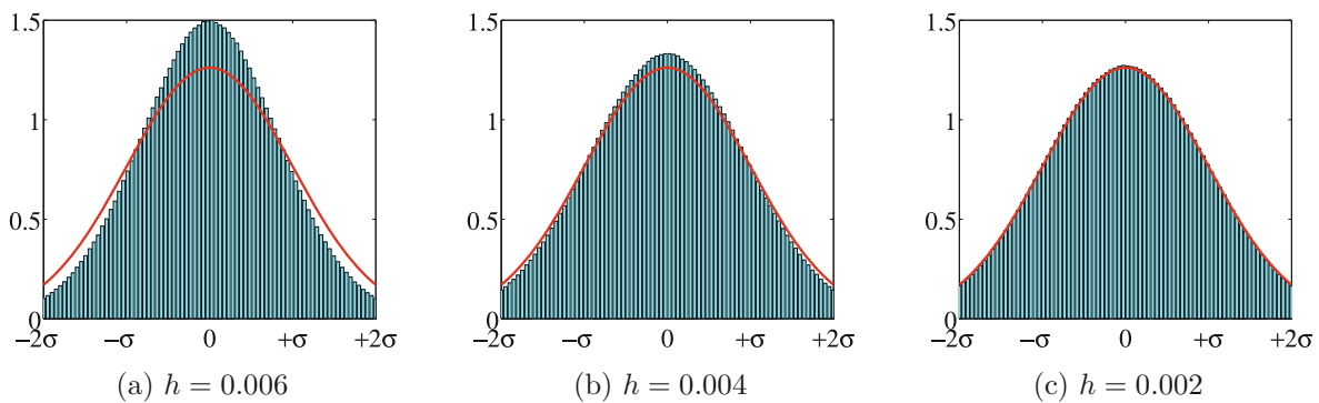
FIGURE 2. Momentum distributions from Hoover-Langevin simulations.
