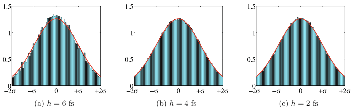
FIGURE 3. Momentum distributions from MANH simulations.
