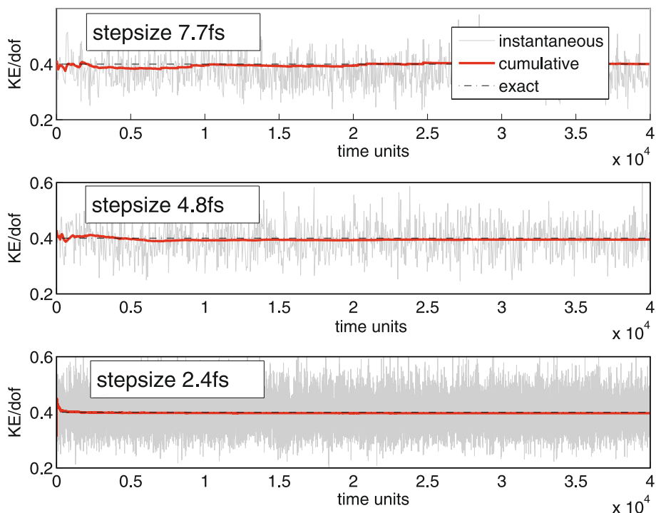
FIGURE 8. Butane-8 simulations. Kinetic energy per degree of freedom (cumulative and instantaneous) graphed against time, for each of three stepsizes using the MANH thermostat. Note the convergence to target temperature.
