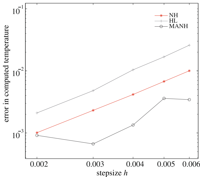
FIGURE 4. Discrepancy of average kinetic energy from temperature for the three methods.
