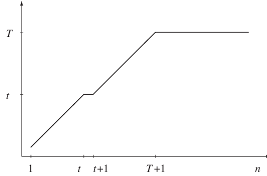
FIGURE 1. Illustration of the sequence (D_n) , where D_n = |w_\beta^{(n)}|_B - |u_\beta^{(n)}|_B . The consecutive values are connected by a line and t := \lfloor \frac{p+q}{q+1} \rfloor and T = \lceil \frac{p-1}{q} \rceil .
