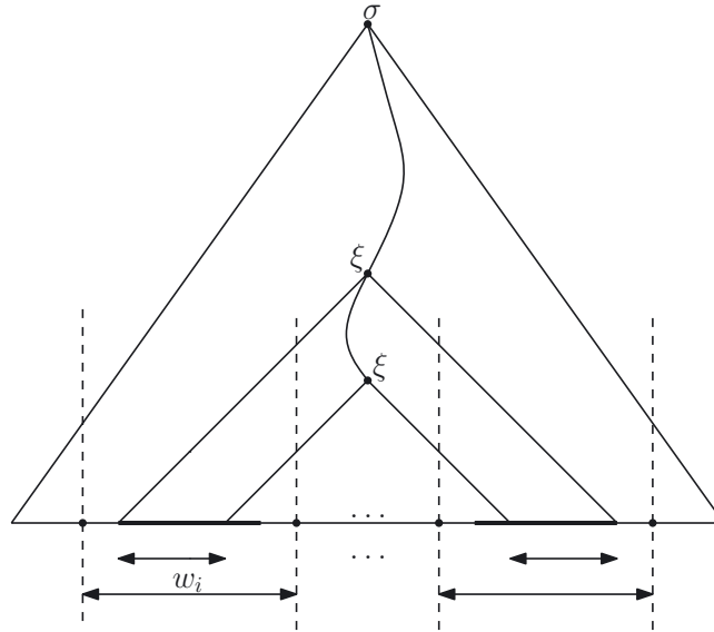
FIGURE 4. A pumpable subword of w_i and its associated subword.
