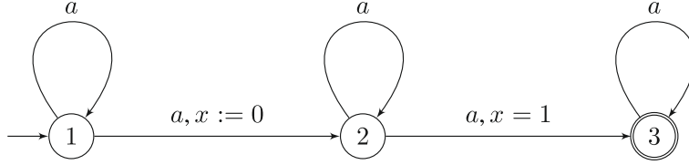
FIGURE 13. A timed automaton whose complement language is not accepted by a timed automaton.
