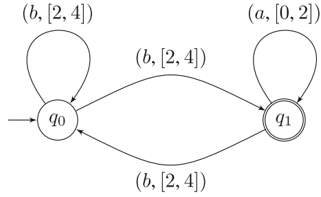
FIGURE 6. An abstract automaton for the expression (1).
