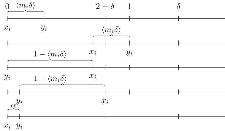
FIGURE 20. The decrement step. Note that \alpha = 2 - \delta - (1 - \langle m_i \delta \rangle) .
