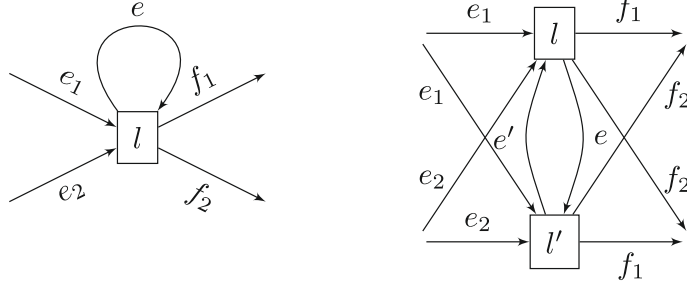
FIGURE 7. Step (a): removing self loops.
