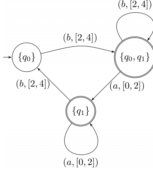
FIGURE 11. A deterministic finite automaton for the expression (1).
