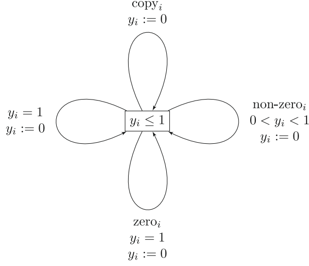
FIGURE 21. The system \mathcal{H}_i^y .
