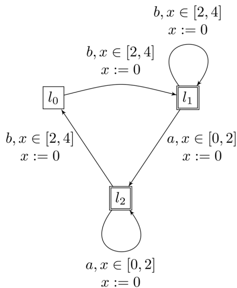
FIGURE 12. A deterministic hybrid system for the expression (1).
