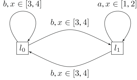
FIGURE 5. An example of a hybrid system.
