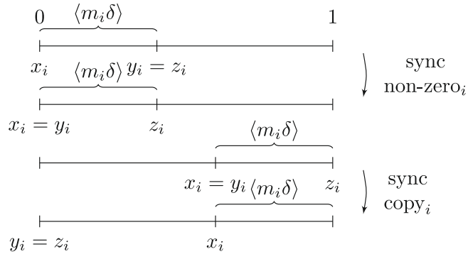
FIGURE 23. Negative zero test.
