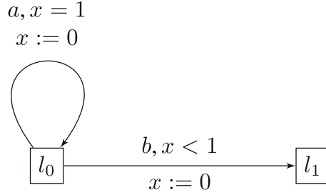
FIGURE 3. A simple hybrid system.
