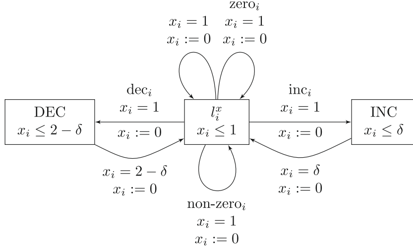
FIGURE 18. The system \mathcal{H}_i^x with \delta = \sqrt{2} .
