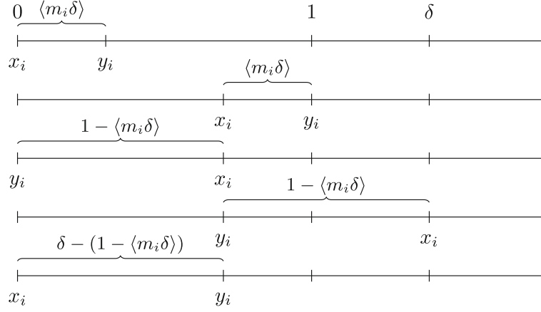
FIGURE 19. The increment step. Note that \delta - (1 - \langle m_i \delta \rangle) = \langle (m_i + 1) \delta \rangle .
