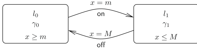
FIGURE 2. Thermostat.
