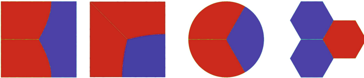
FIGURE 17. Candidates for the minimal 3-partitions.
