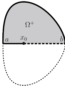
FIGURE 9. Dirichlet-Neumann problem.
