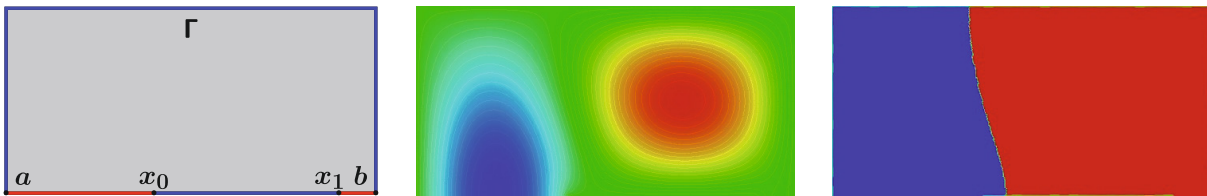
FIGURE 16. Eigenmodes for the Neumann-Dirichlet-Neumann problem on the half-square. Left: the domain; center: the second eigenfunction; right: the associated nodal domains.
