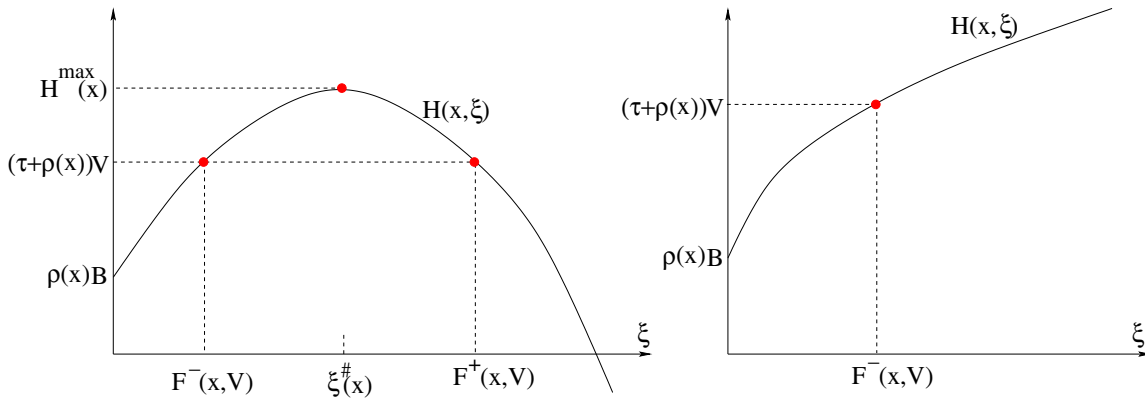
FIGURE 2. Left : the case where x < x^* . For (r + \rho(x))V > H^{\max}(x) the equation (3.3) has no solution. At a point where (r + \rho(x))V < H^{\max}(x) , it determines two distinct values F^-, F^+ for V' . Right : the case where x > x^* . For any (r + \rho(x))V > \rho(x)B , the equation (3.3) determines a unique solution V' = F^-(x, V) .
