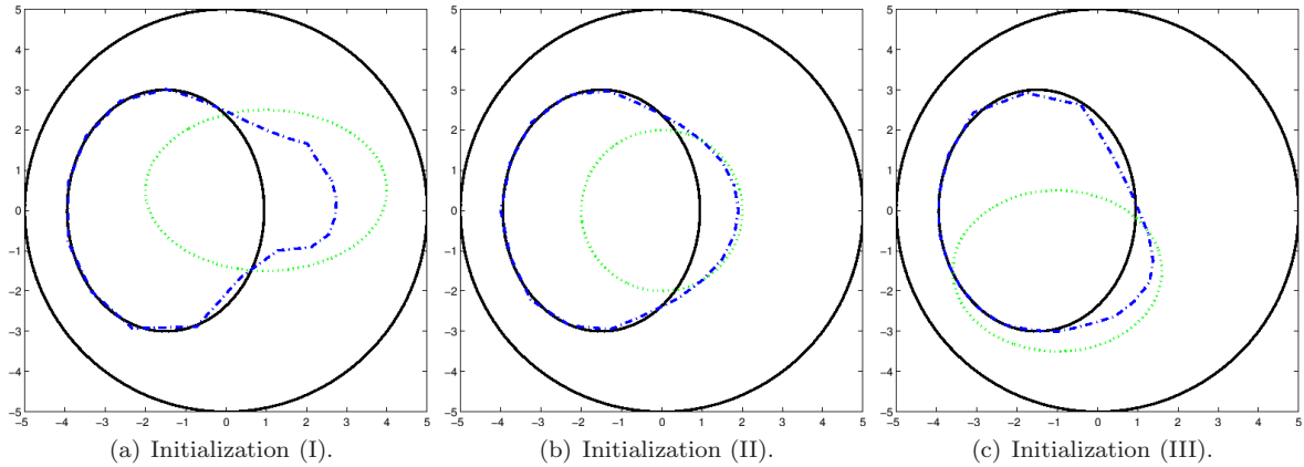
FIGURE 7. Certified Descent Algorithm using multiple measurements for different initial configurations. Initial configuration ( dotted green ), target inclusion ( solid black ) and reconstructed interface ( dashed blue ). (color online)
