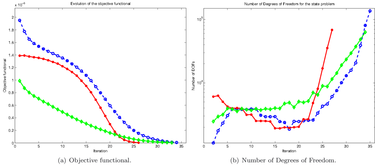
FIGURE 8. Certified Descent Algorithm using multiple measurements for initial guess (I) blue circles ; (II) red stars ; (III) green diamonds . (a) Evolution of the objective functional. (b) Number of Degrees of Freedom. (color online)
