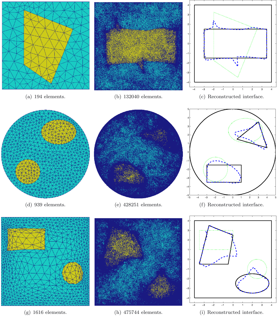
FIGURE 9. Certified Descent Algorithm using multiple measurements: test cases (i)–(iii). Left : Initial mesh. Center : Final mesh. Right : Initial configuration ( dotted green ), target inclusion ( solid black ) and reconstructed interface ( dashed blue ). (color online)
