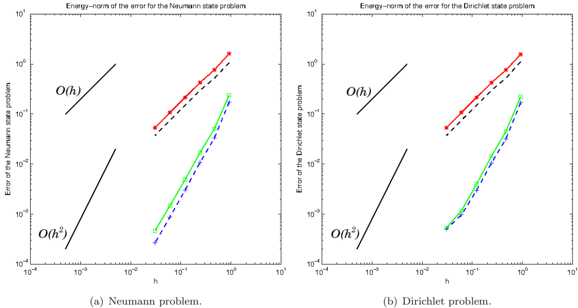
FIGURE 2. Comparison of the convergence rates with respect to the mesh size h for the (a) Neumann and (b) Dirichlet state equations. Analytical errors using \mathbb{P}^1 (black dash) and \mathbb{P}^2 (blue cross) Lagrangian Finite Element functions; error estimates based on the complementary energy principle using \mathbb{P}^1 (red star) and \mathbb{P}^2 (green square) Lagrangian Finite Element functions. (color online)
