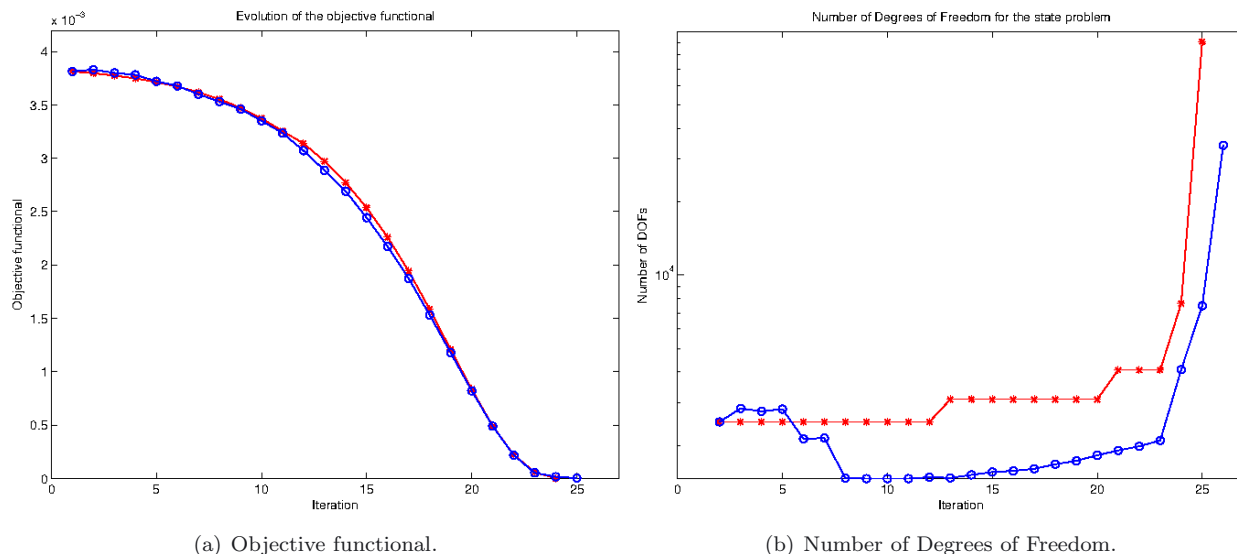
FIGURE 5. Comparison of 1-mesh ( red star ) and 2-mesh ( blue circle ) reconstruction strategies. (a) Evolution of the objective functional. (b) Number of Degrees of Freedom. (color online)
