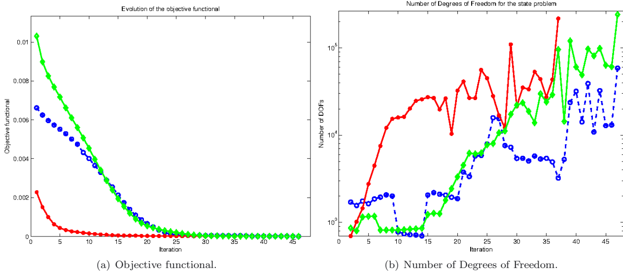
FIGURE 10. Certified Descent Algorithm using multiple measurements: Test case (i) blue circles ; (ii) red stars ; (iii) green diamonds . (a) Evolution of the objective functional. (b) Number of Degrees of Freedom. (color online)
