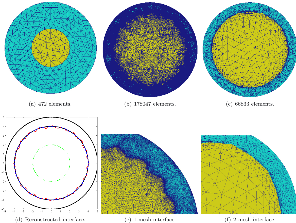
FIGURE 4. Comparison of 1-mesh and 2-mesh reconstruction strategies. (a) Initial mesh. (b) Final mesh using 1-mesh strategy. (c) Final mesh using 2-mesh strategy. (d) Initial configuration ( dotted green ), target inclusion ( solid black ) and reconstructed interfaces using 1-mesh ( dot-dashed red ) and 2-mesh ( dashed blue ) strategies. (e) Zoom of the reconstructed interface using 1-mesh strategy. (f) Zoom of the reconstructed interface using 2-mesh strategy. (color online)
