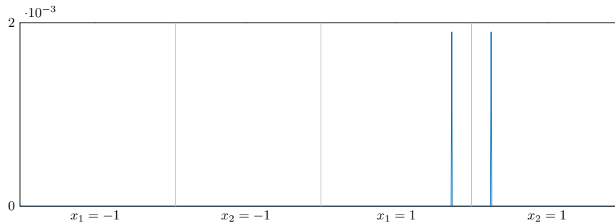
FIGURE 3. Optimal Neumann boundary control \bar{u}_h for desired state in Figure 1a.
