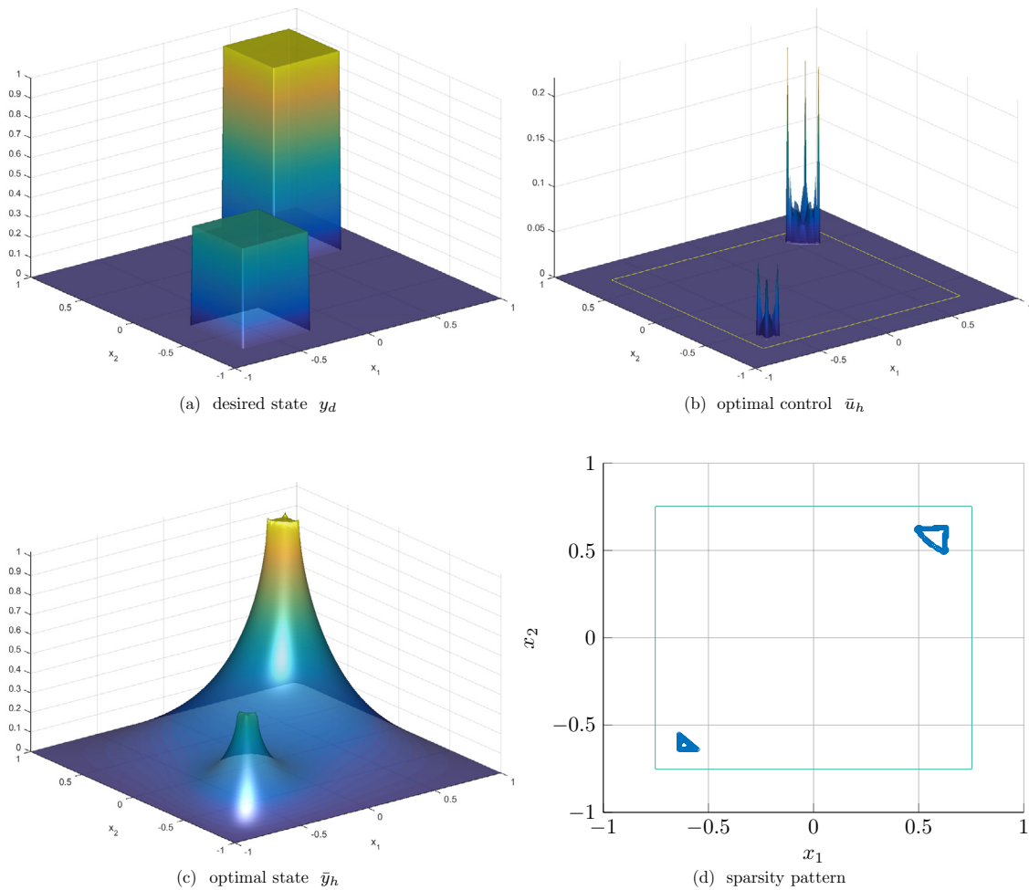
FIGURE 1. First desired state and resulting optimal control and state.
