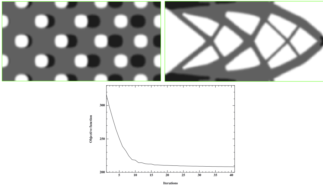
FIGURE 23. Initialization with two materials (top left), optimal shape (top right) and convergence history of the objective function (bottom).
