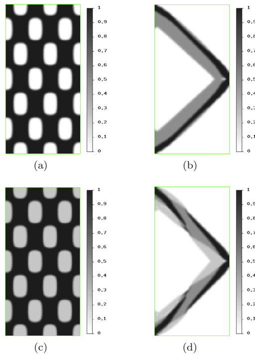
FIGURE 16. Short cantilever using two or three phases and void; (a) initialization for two phases and void, (b) optimal shape for two phases and void, (c) initialization for three phases and void, (d) optimal shape for three phases and void.
