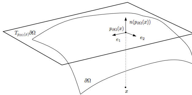
FIGURE 4. Principal directions, normal vector at the projection point of x \in \mathbb{R}^d .
