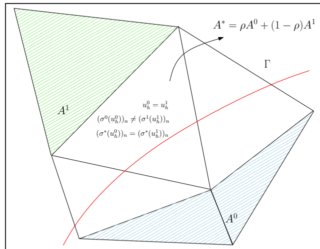
FIGURE 2. Transmission condition in a fixed mesh framework.
