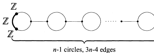
Fig. 8. A (3n - 5) -dimensional simplex in \mathcal{M}_n .
