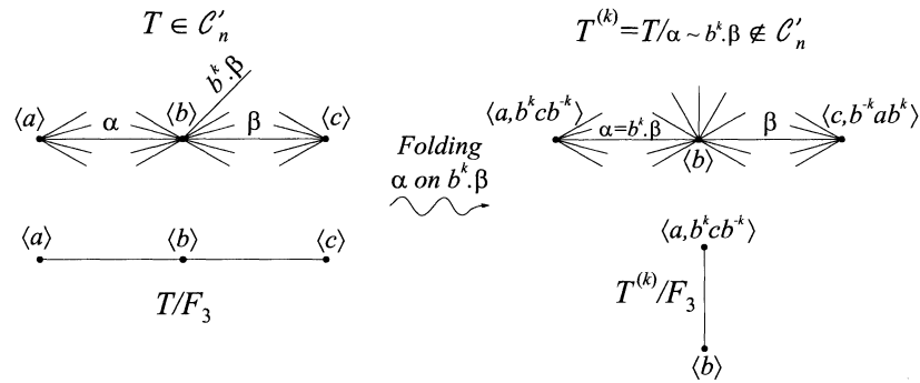
Fig. 3. T \in \mathcal{C}'_n is approximated by T^{(k)} = T/\alpha \sim w_k \cdot \beta \notin \mathcal{C}'_n . \mathcal{C}'_n is not open in \overline{CV}_n for n \geq 3 .
