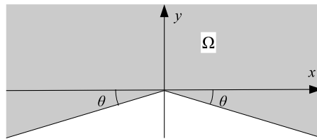
Fig. 1. The conical domain \Omega in the two-dimensional case ( d = 1 ).
