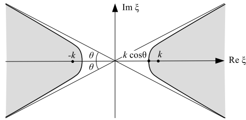
Fig. 2. Domains of analyticity of \hat{\varphi} .
