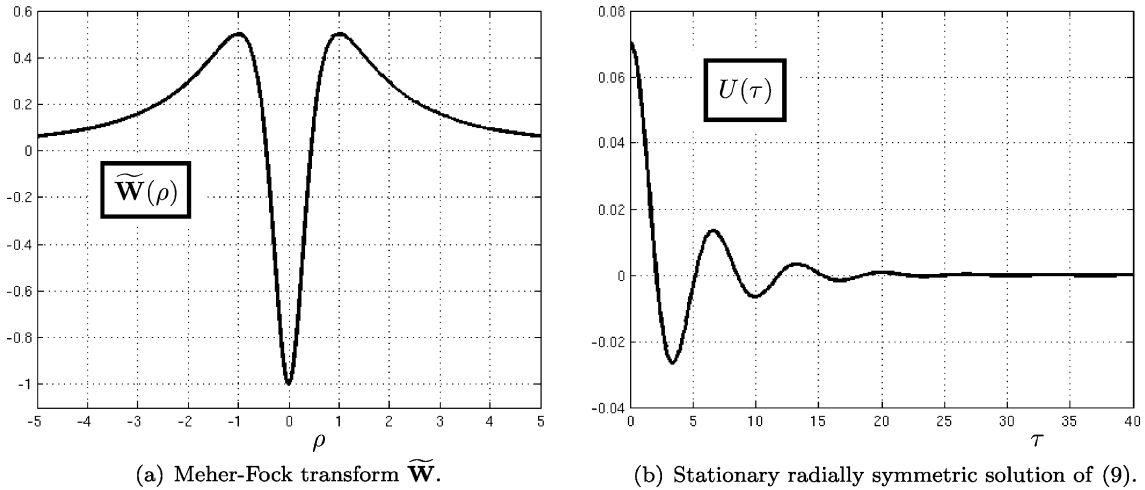
Fig. 1. Left. Plot of \tilde{W} as a function of \rho , the value of the parameters are \alpha_1 = 3, \alpha_2 = 4/3, a_1 = 1 and a_2 = \sqrt{3}/3 . Right. Plot of a stationary radially symmetric solution of (9) obtained by solving (17).
