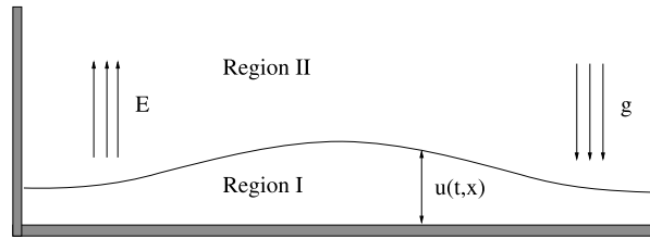
Fig. 1. A viscous thin film submitted to an electric field \mathbf{E} and gravity g .
